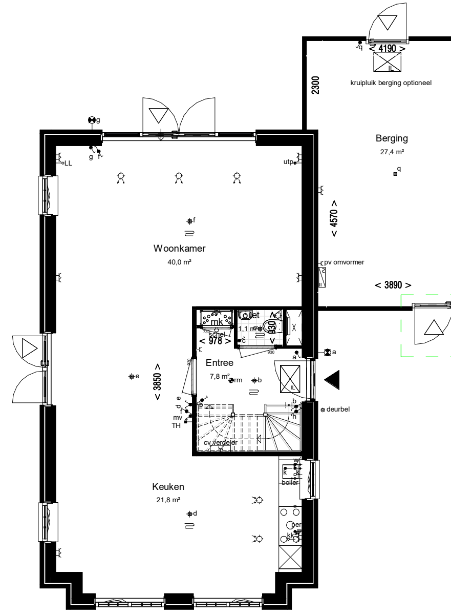
Begane grond, PEIL=0
